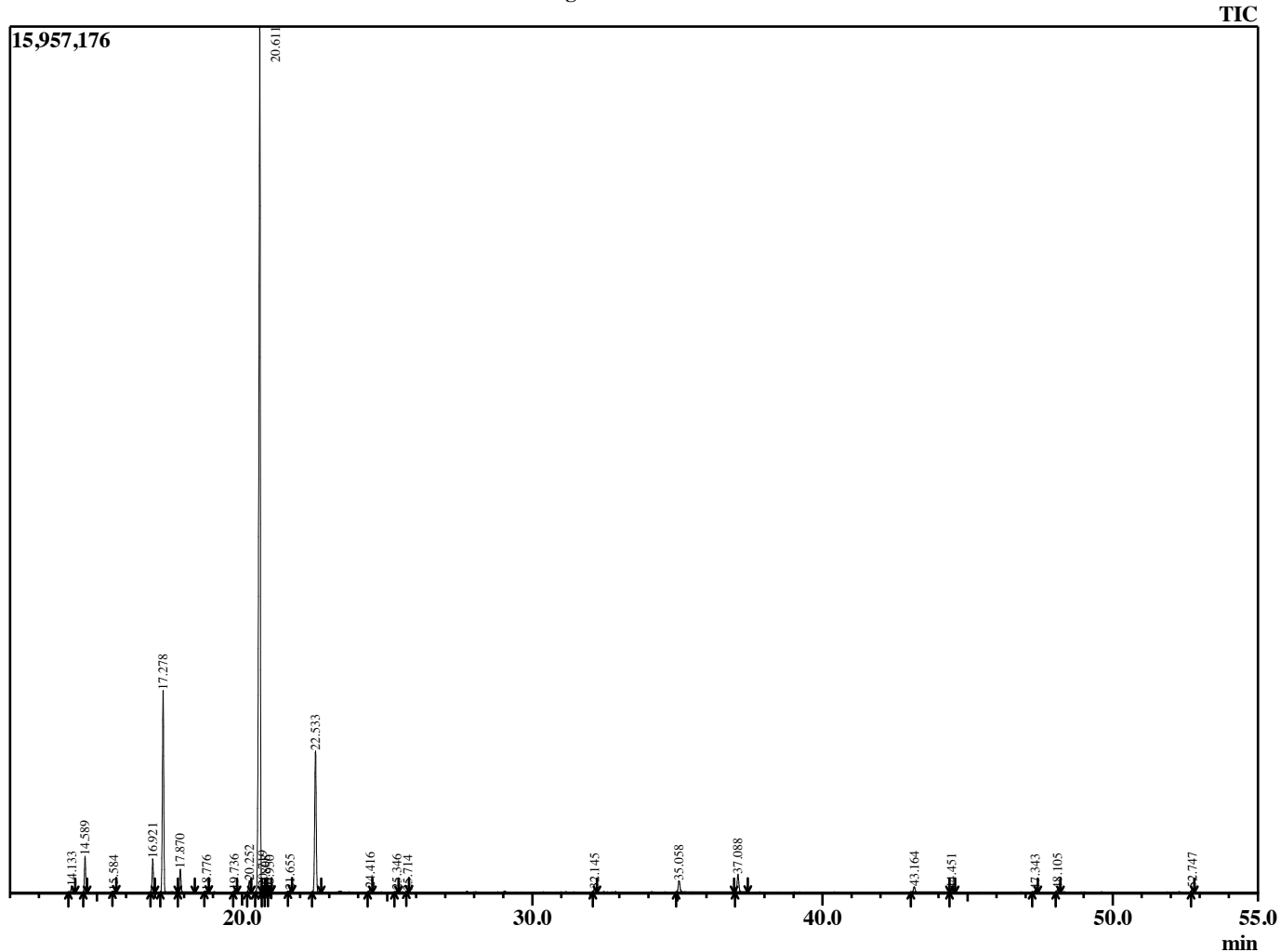
Chromatogram CitLim2 Lot 16400
